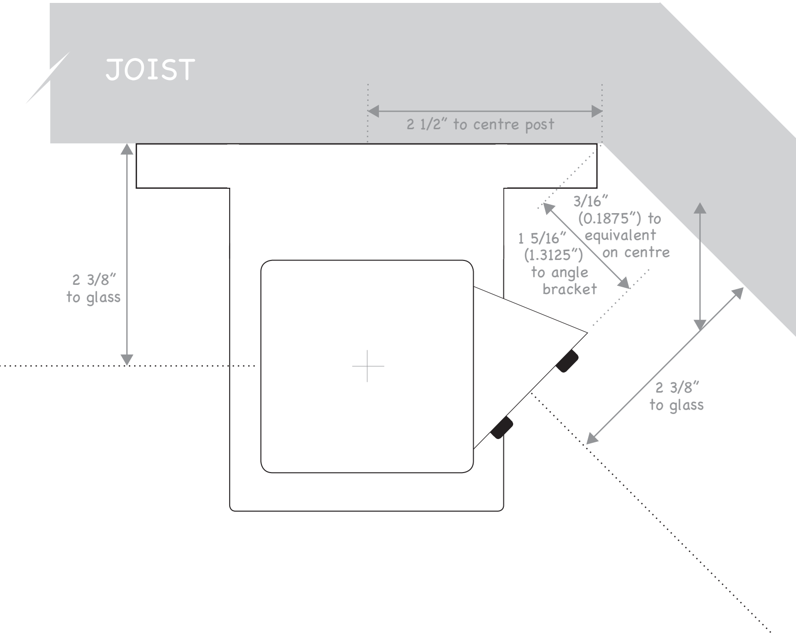
VistaPost fascia -- inside 45° w/Lite 10 connectors
